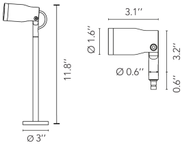
LANDLORD SPOT 300 MM H / 11.8 IN H / Ø 40 MM
